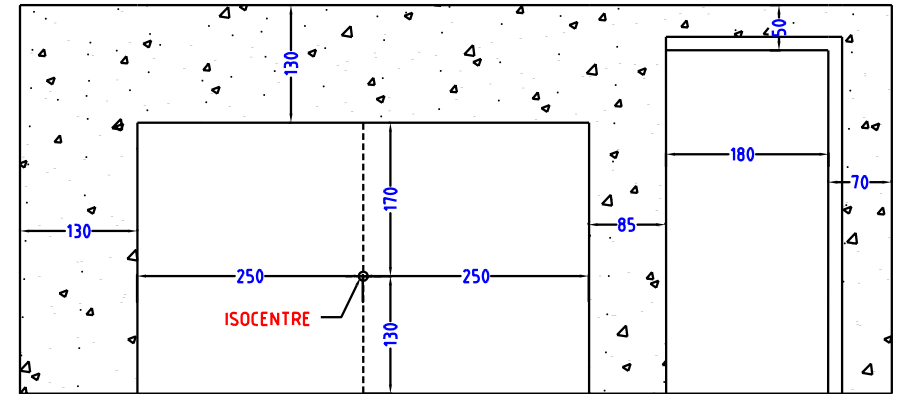
SECTION X-X
