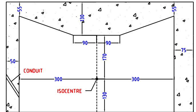
SECTION Y-Y
